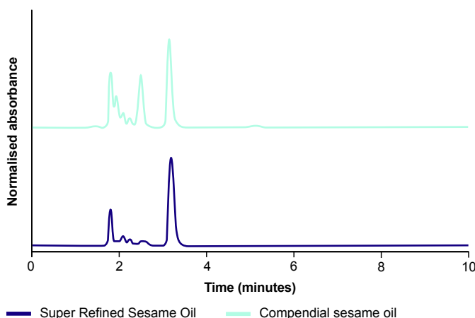
Figure 1: Chromatogram of haloperidol decanoate in sesame oil after 12 weeks at 40°C
