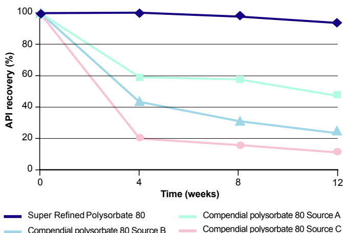
Figure 3: % docetaxel recovery in polysorbate 80 at 40°C
