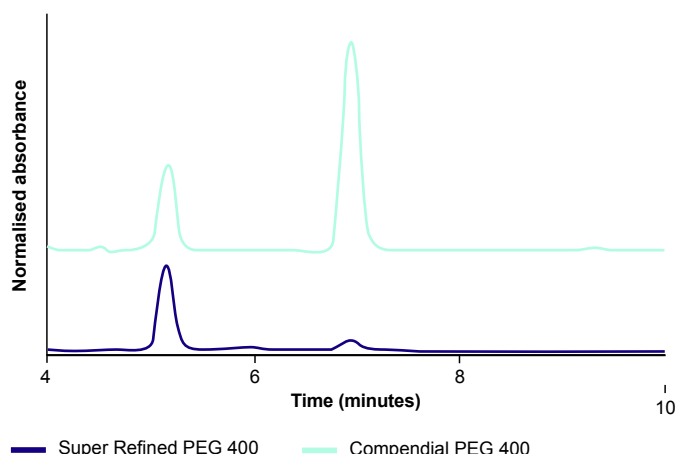
Figure 2: Chromatogram of fulvestrant in PEG 400 after 12 weeks at 40°C
